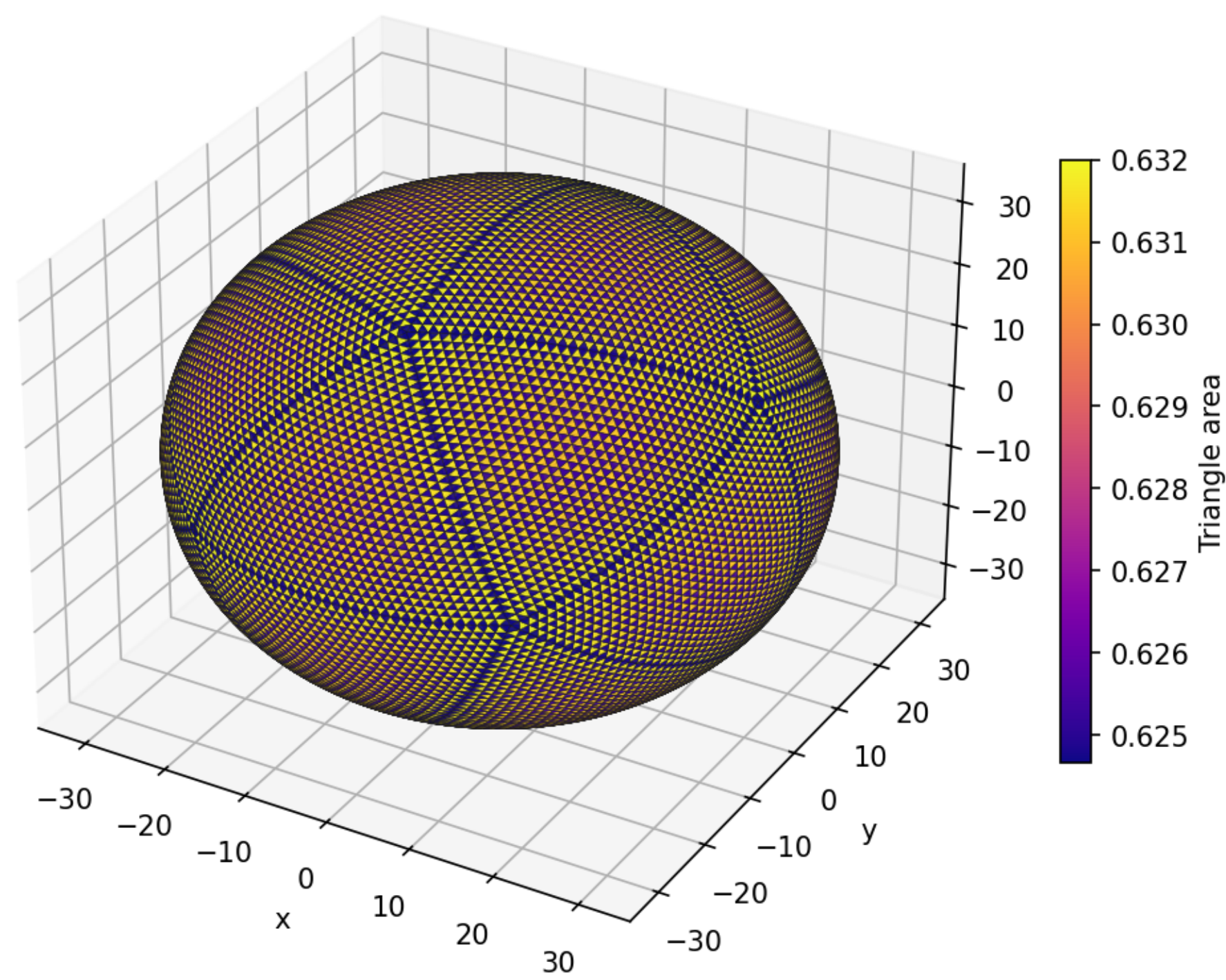
Primal mesh - triangle area
