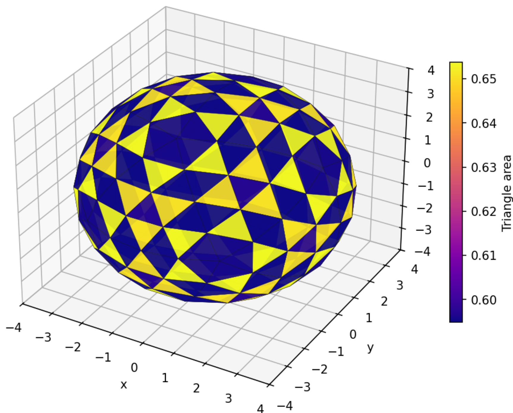
Primal mesh - triangle area
