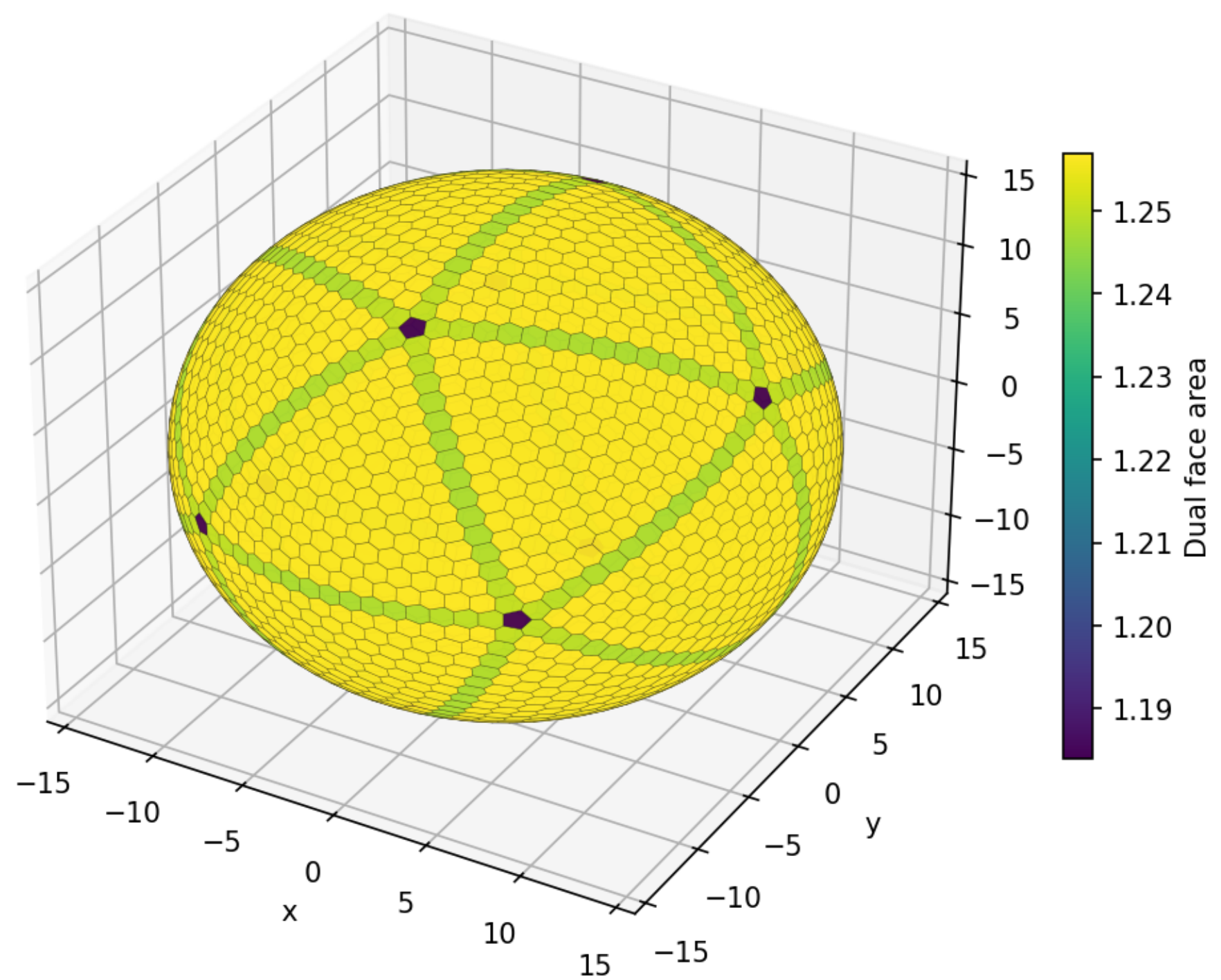
Dual mesh - face area
