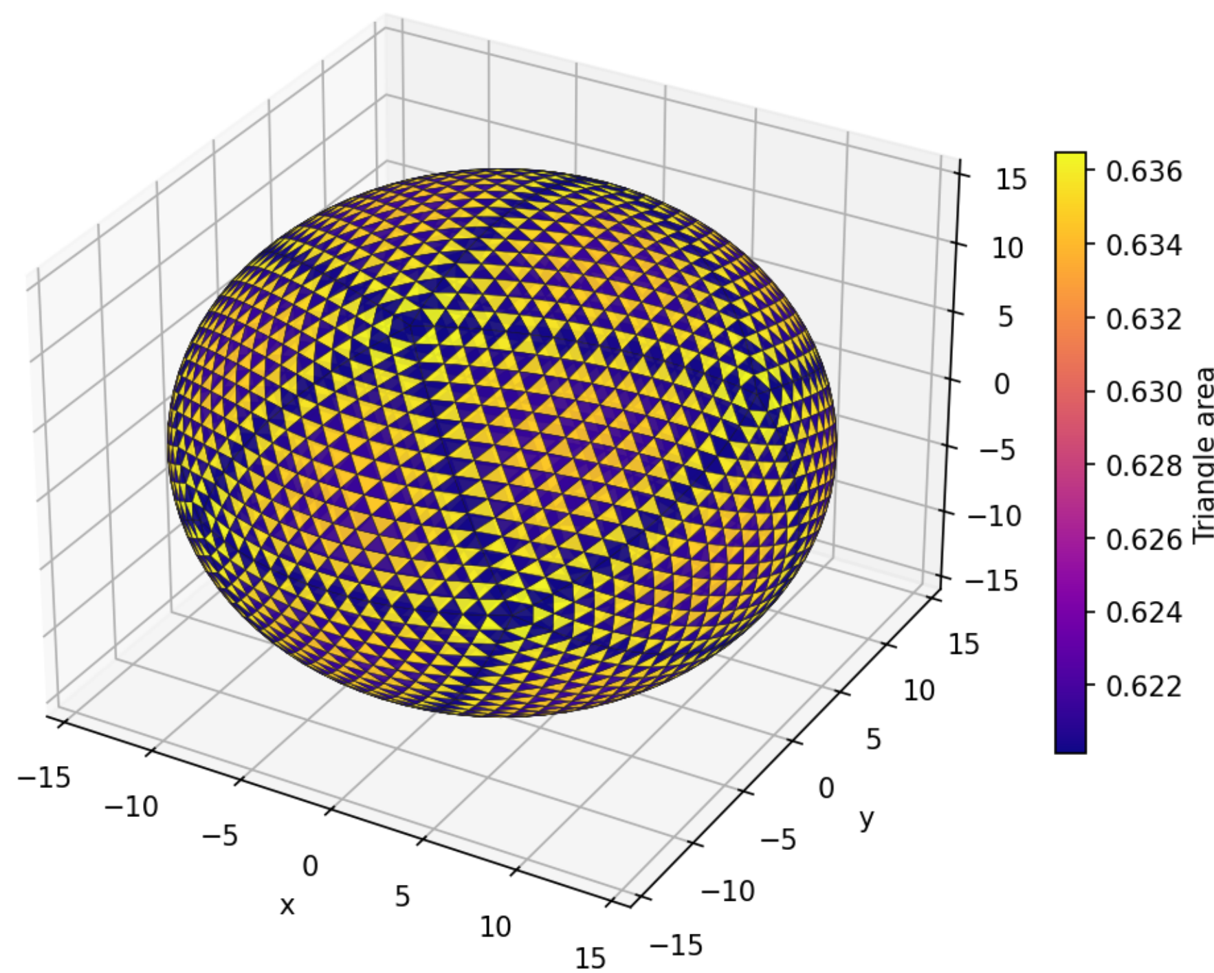
Primal mesh - triangle area
