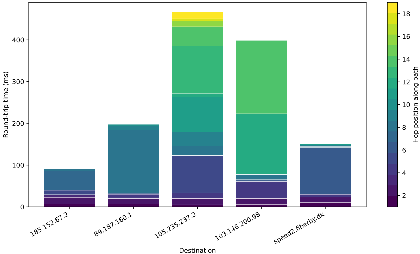
Per-hop incremental latency breakdown (traceroute)
