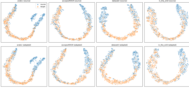
Fig. 3. t-SNE of 750 source + 750 target embeddings for all four targets (columns), before (top row) vs. after adaptation (bottom row); blue=source, orange=target. In every panel, source and target intermix within each of the two class-structured arcs rather than separating into domain-specific clusters, both before and after adaptation—matching the proxy \mathcal{A} -distance result that domain separability is not reduced by adaptation (Table IX).
