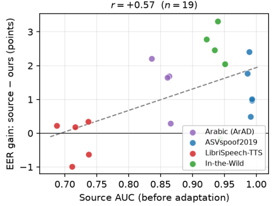
Fig. 2. EER gain (source—ours) vs. source AUC before adaptation, one point per (target, seed), all 19 leave-one-corpus-out runs (5 seeds per target, 4 for Arabic). The positive trend ( r=+0.57 ) supports the ranking-precondition account of Sec. III-C: LibriSpeech-TTS (red), the lowest-AUC target, clusters at or below zero gain, while the higher-AUC targets cluster above it—the relationship strengthened, rather than weakened, when the seed count grew from 3 to 5 per target ( r from +0.41 at n=12 to +0.57 at n=19 ), though one LibriSpeech-TTS seed still shows a small negative gain even relative to its own AUC.
