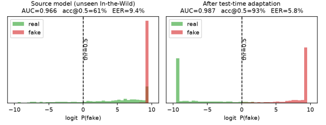
Fig. 1. Detector scores on unseen In-the-Wild audio. Left : the source model pushes many real clips past \tau=0.5 (accuracy well below AUC) yet still ranks most real below fake. Right : TTA shifts the real mass back across the threshold.
