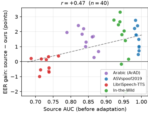
Fig. 2. EER gain (source—ours) vs. source AUC before adaptation, one point per (target, seed), all 40 runs. LibriSpeech-TTS (red), the lowest-AUC target, clusters at or below zero gain; higher-AUC targets cluster above it ( r=+0.47 , p=0.002 ).
