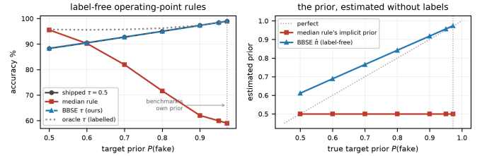
Fig. 2. The same official-DF score distribution, resampled to a range of target priors. Left: the median rule is the best label-free operating-point rule at 50/50 — the only prevalence at which our earlier threshold-control experiments ever measured it, because the evaluation pipeline balanced every pool to 0.489–0.539 — and the worst by 40 points at the benchmark’s own prior. Right: what the two rules assume about the prior. The median rule’s implicit estimate is a flat 0.5; BBSE tracks the truth, with a positive bias that is largest at balanced priors (it assumes label shift, and DF’s codec conditions also shift covariates) and vanishes as the prior approaches the one the benchmark has.
