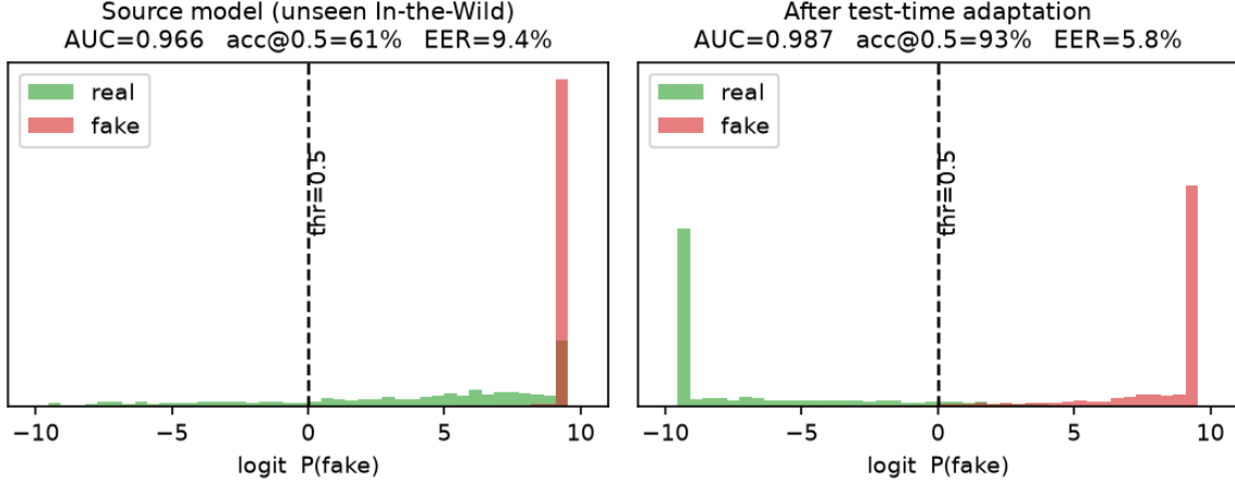
Fig. 1. Detector scores (logit axis; scores concentrate near the extremes) for real vs. fake clips on the unseen In-the-Wild corpus (representative seed from preliminary analysis). Left: the source model pushes many real clips past the 0.5 threshold (accuracy at \tau=0.5 well below AUC) yet still ranks most real below fake. Right: unsupervised test-time adaptation shifts the real mass back across the threshold, raising both accuracy@0.5 and AUC. Tables II–III report the full 5-seed (4 for Arabic), 4-target means used for all headline claims in this paper.
