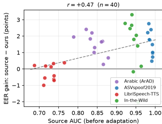
Fig. 2. EER gain (source—ours) vs. source AUC before adaptation, one point per (target, seed), all 40 leave-one-corpus-out runs (10 seeds per target). The positive trend ( r=+0.47 , p=0.002 ) supports the ranking-precondition account of Sec. III-C: LibriSpeech-TTS (red), the lowest-AUC target, clusters at or below zero gain, while the higher-AUC targets cluster above it—the relationship survived the seed count growing from 3 to 10 per target, at a somewhat smaller coefficient ( r from +0.41 at n=12 to +0.47 at n=40 , now with p=0.002 ), though one LibriSpeech-TTS seed still shows a small negative gain even relative to its own AUC.
