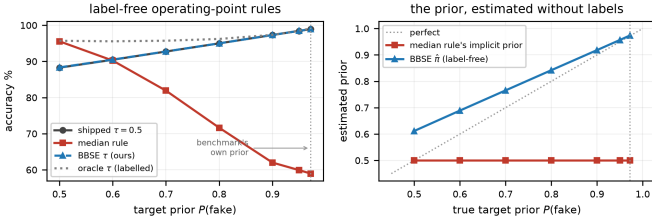
Fig. 2. The same official-DF score distribution, resampled to a range of target priors. Left: the median rule is the best label-free operating-point rule at 50/50 — the only prevalence at which our earlier threshold-control experiments ever measured it, because the evaluation pipeline balanced every pool to 0.489–0.539 — and the worst by 40 points at the benchmark’s own prior. Right: what the two rules assume about the prior. The median rule’s implicit estimate is a flat 0.5; BBSE tracks the truth, with a positive bias that is largest at balanced priors (it assumes label shift, and DF’s codec conditions also shift covariates) and vanishes as the prior approaches the one the benchmark has.
