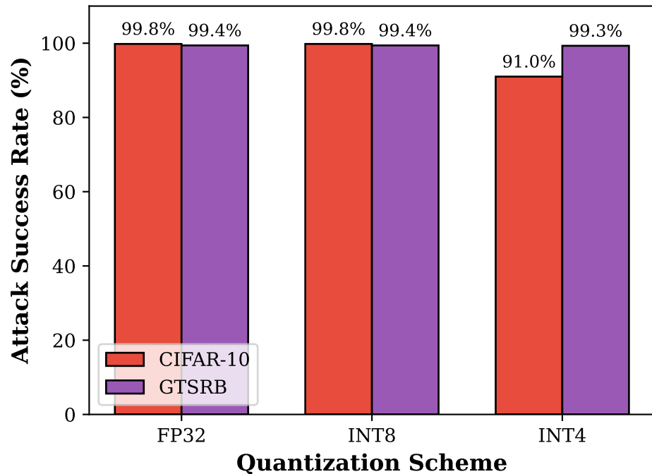
Backdoor Persistence Under Quantization
