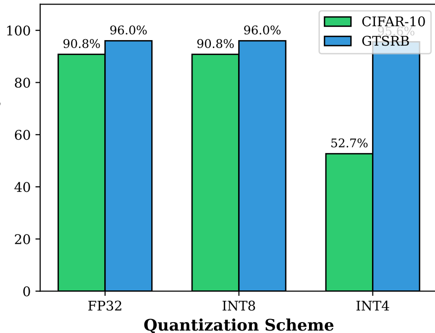
Model Accuracy Under Quantization
