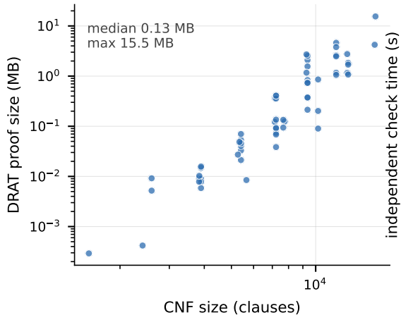
(a) Refutation certificates stay small
