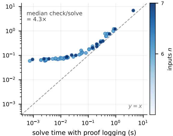
(b) Checking costs a small multiple of solving
