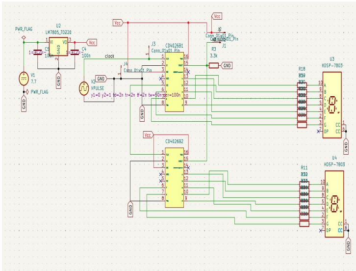
Figure 1: Circuit Schematic
