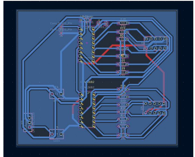
Figure 2: PCB Layout
