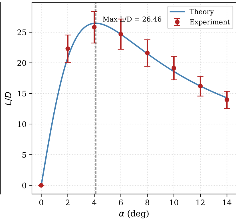
Lift-to-drag ratio
