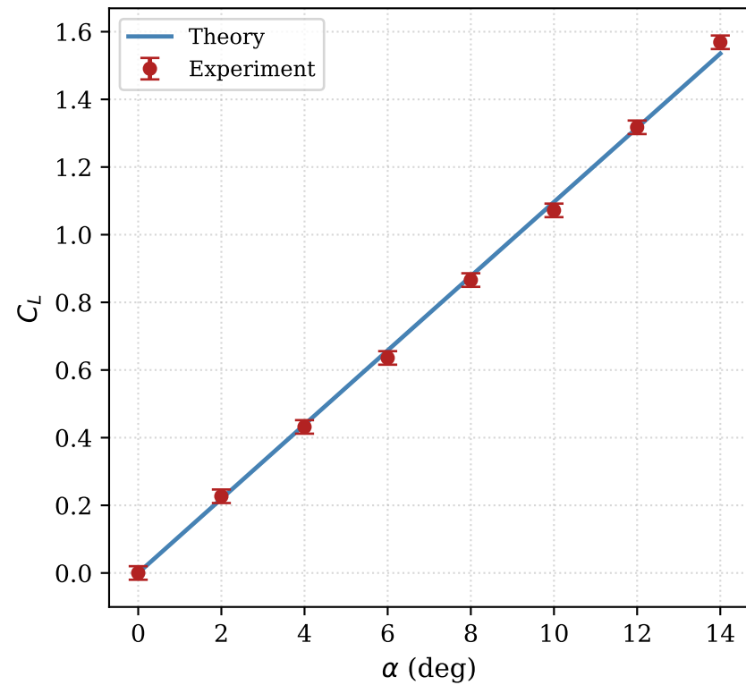
Lift curve
