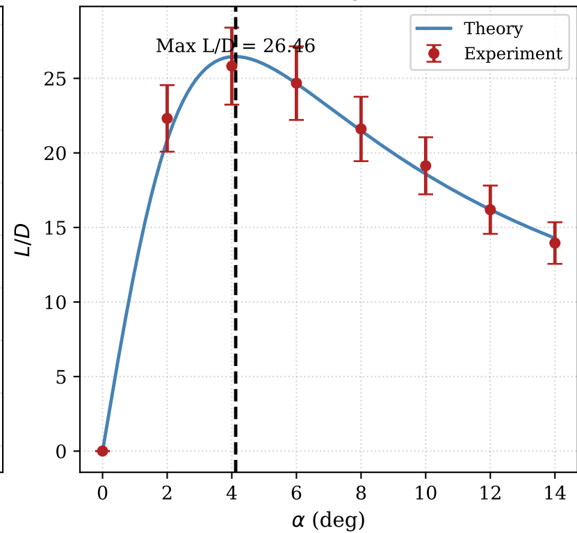
Lift-to-drag ratio
