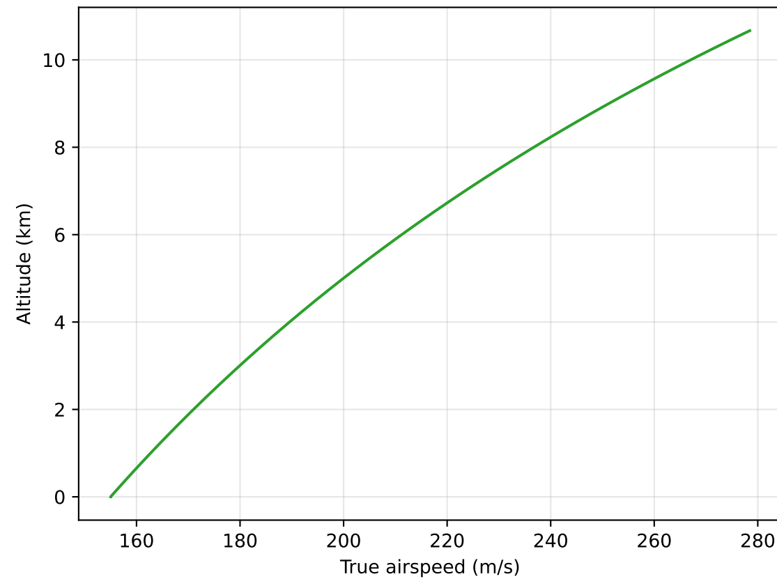
Climb performance, sea level to FL350
