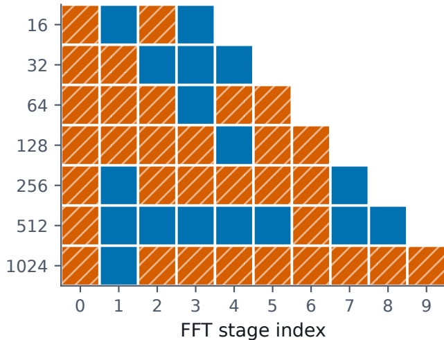
(a) Multiplier precision
