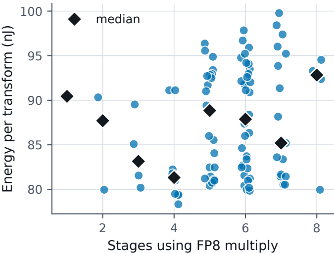
(a) Energy vs FP8 stages
