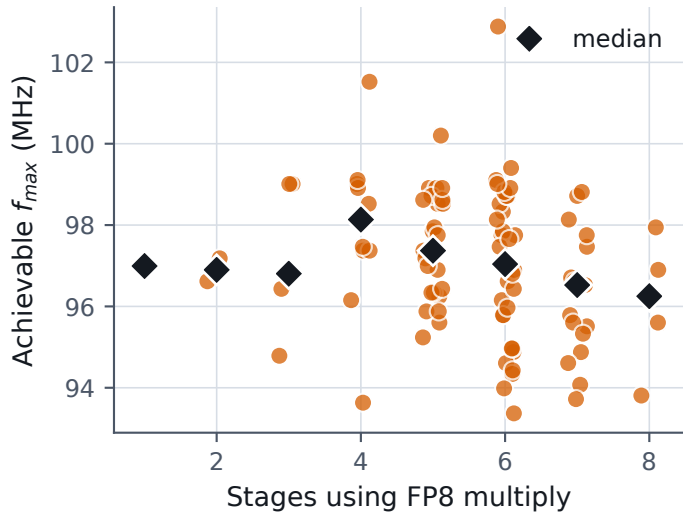
(b) f_{max} vs FP8 stages
