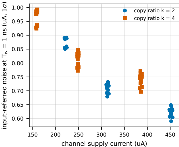
72 sizing/bias points: lower noise costs power, not area
