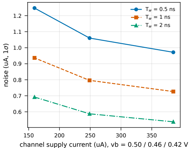
chosen sizing ( k = 4 , W1 = 15 \mu\text{m} , \text{OTA1 } 8 \mu\text{m} , mirror 16/0.36 \mu\text{m} )
