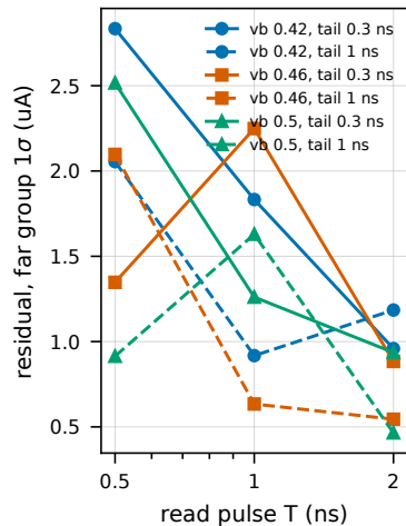
calibrated on the real transient
