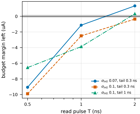
g = 8 , vb 0.50, \Delta T 5 K (grey: Monte-Carlo scatter)
