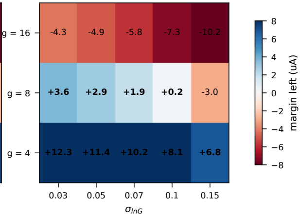
8 mV rail droop
