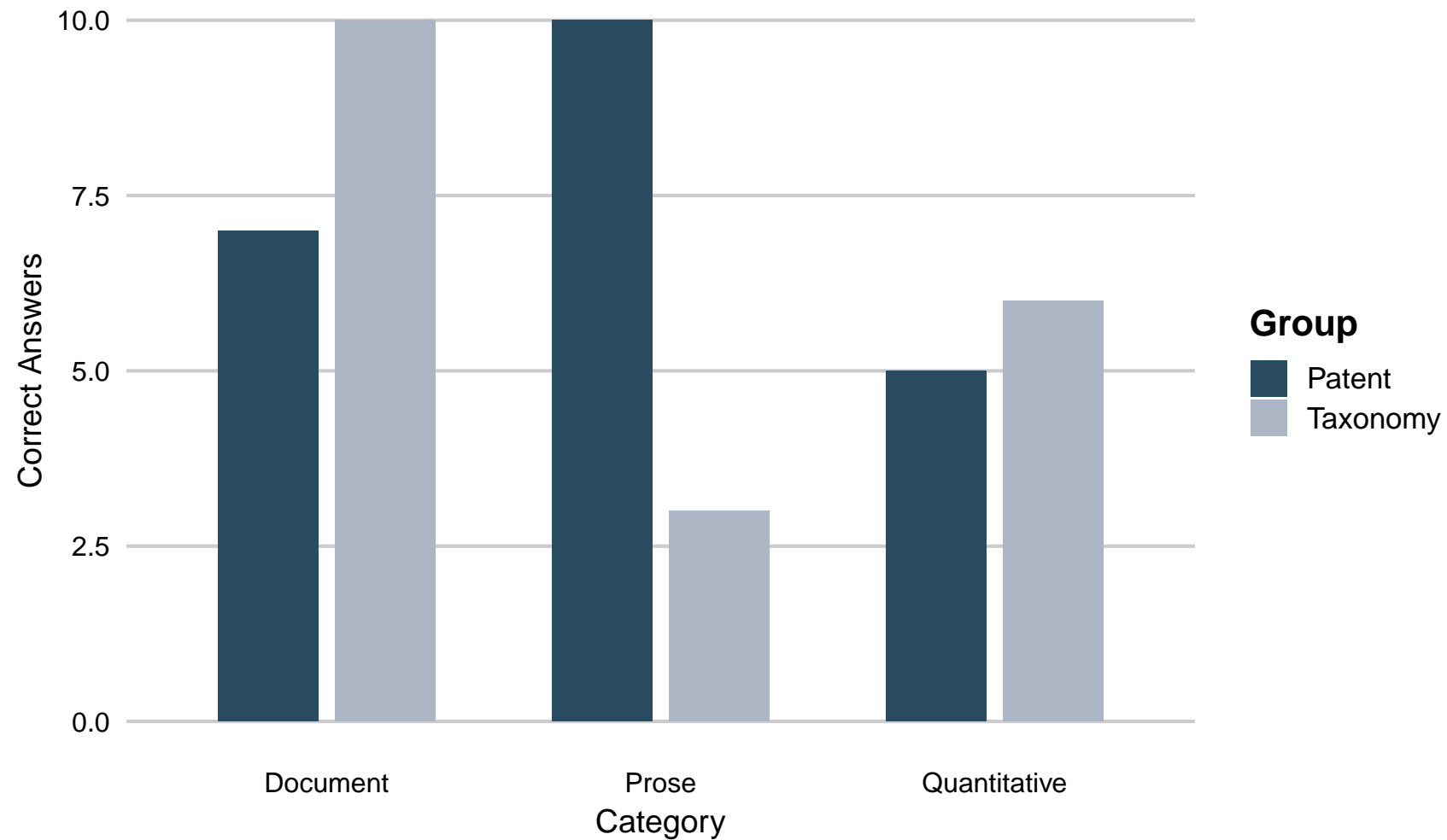
Taxonomy vs Patent: Accuracy by Category
