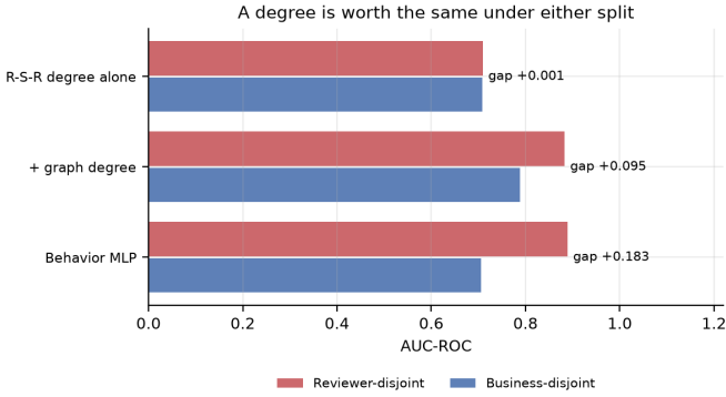
Fig. 4. What the split does and does not reach. Behavioral features lose 0.183 AUC when businesses stop spanning the split; the same features plus two graph degrees lose 0.095; a graph degree on its own loses 0.001. The split partitions rows, and a degree is not computed from rows it can partition.
