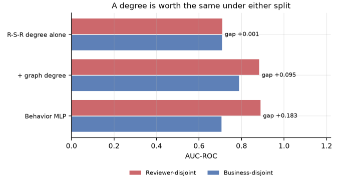
Fig. 8. What the split does and does not reach. Behavioral features lose 0.183 AUC when businesses stop spanning the split; the same features plus two graph degrees lose 0.095; a graph degree on its own loses 0.001. The split partitions rows, and a degree is not computed from rows it can partition.
