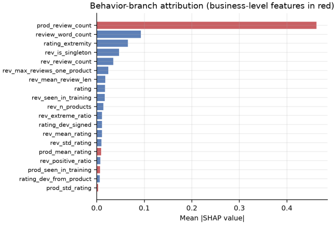
Fig. 9. Mean absolute SHAP value per behavioral feature for the behavior-only MLP. Business-level features are shown in red. The single most influential feature is how many reviews a business has received, which carries no information about the review being classified.
