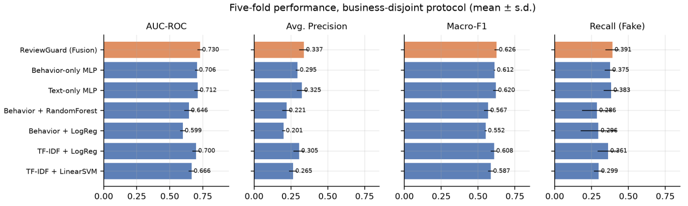
Fig. 3. Five-fold performance under the business-disjoint protocol. Error bars are standard deviations across folds.
