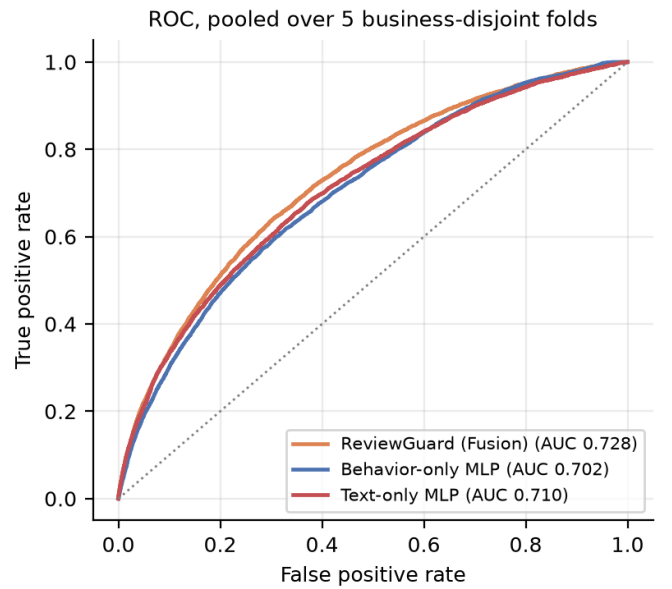
Fig. 5. ROC curves for ReviewGuard and its two ablations, pooled over the out-of-fold predictions of all five business-disjoint folds.
