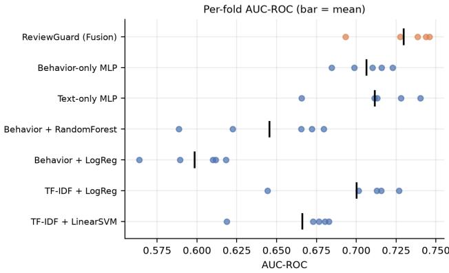
Fig. 4. Per-fold AUC-ROC under the business-disjoint protocol. Horizontal bars mark per-model means. Fold-to-fold spread is comparable to the differences between the leading models, which is why we decline to claim a fusion win.
