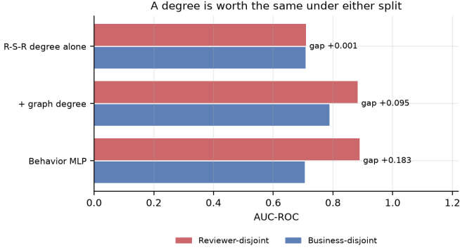
Fig. 8. What the split does and does not reach. Behavioral features lose 0.183 AUC when businesses stop spanning the split; the same features plus two graph degrees lose 0.095; a graph degree on its own loses 0.001. The split partitions rows, and a degree is not computed from rows it can partition.
