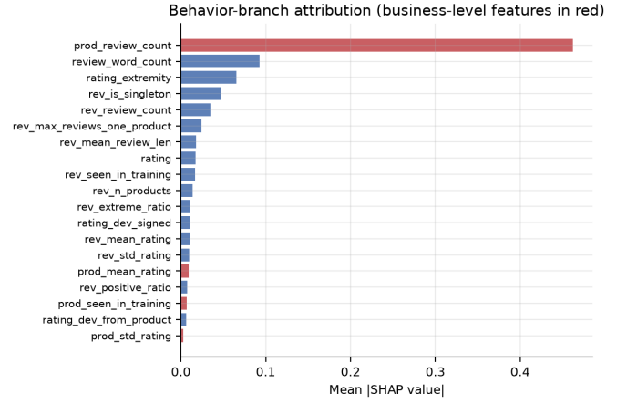
Fig. 9. Mean absolute SHAP value per behavioral feature for the behavior-only MLP. Business-level features are shown in red. The single most influential feature is how many reviews a business has received, which carries no information about the review being classified.
