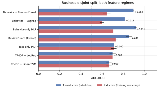
Fig. 7. The business-disjoint split under both feature regimes, ordered by the gain. The three text-based models move by exactly zero — they consume no business aggregates, so the regime cannot reach them — while every behavioral model moves by more than 0.2. One axis, one family.
