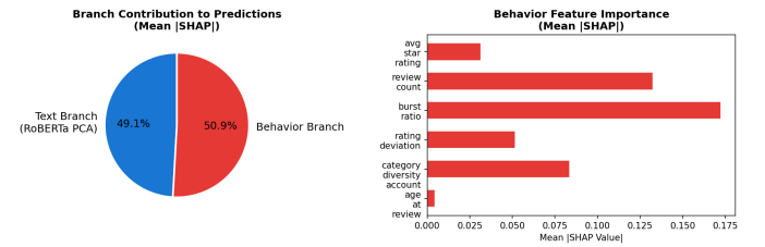
Fig. 5. SHAP feature importance for the ReviewGuard fusion model. Features spanning both behavioral and content dimensions contribute to predictions.
