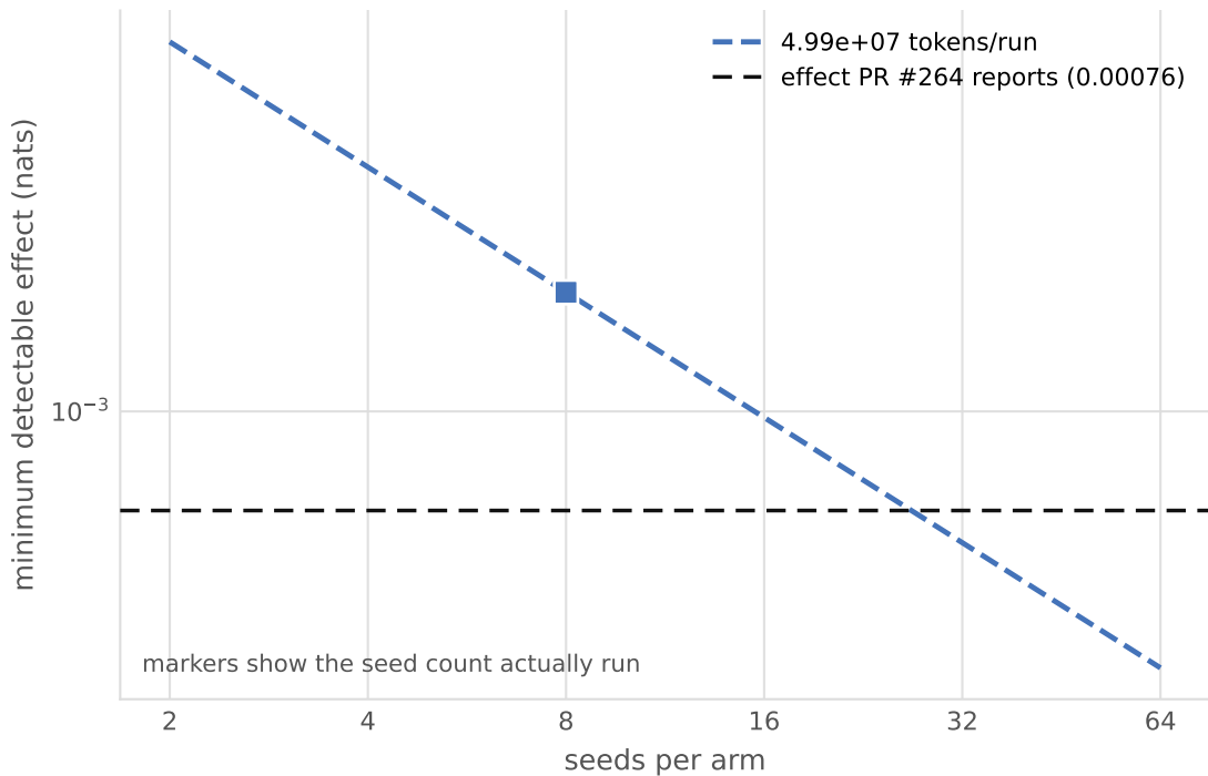
Figure 7 Power: MDE vs seeds, by token budget
