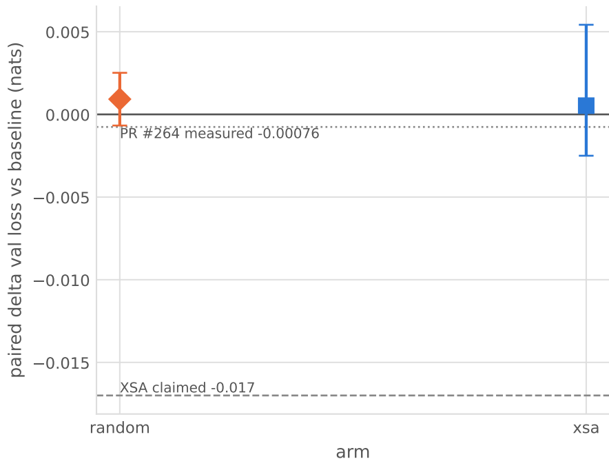
Figure 2. Paired delta loss, 95% CI (n = 4 seeds)
