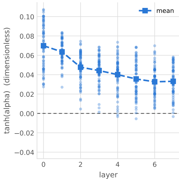
Figure 1 Learned gate per layer and head (n = 16 runs)
