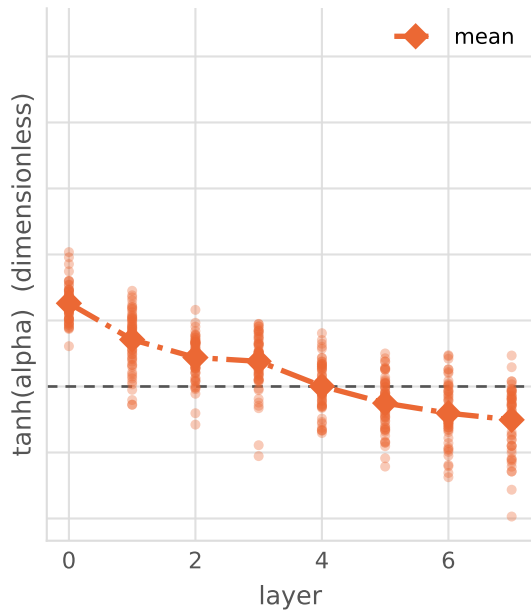
Figure 1 Learned gate per layer and head (n = 16 runs)
