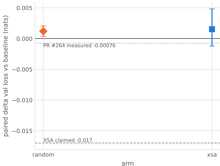
Figure 2 Paired delta loss, 95% CI (n = 8 seeds)
