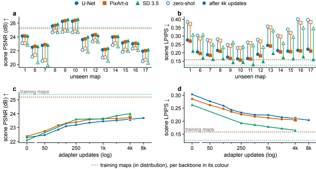
Figure 3: The shift and its repair, per unseen map and per backbone. (a) Scene PSNR and (b) LPIPS zero-shot (open) to 4k adapter updates (filled) for the U-Net, PixArt- \alpha and SD 3.5, with each backbone’s in-distribution level on the training maps (dashed); (c, d) medians over the 13 unseen maps against updates.
