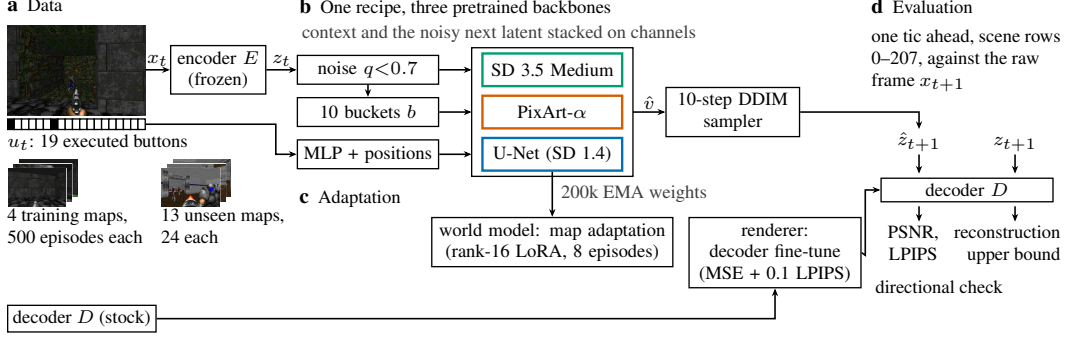
Figure 2: What we built: (a) the benchmark, (b) three backbones under one recipe, (c) adaptation, (d) evaluation against the raw ground-truth frame and the reconstruction upper bound.
