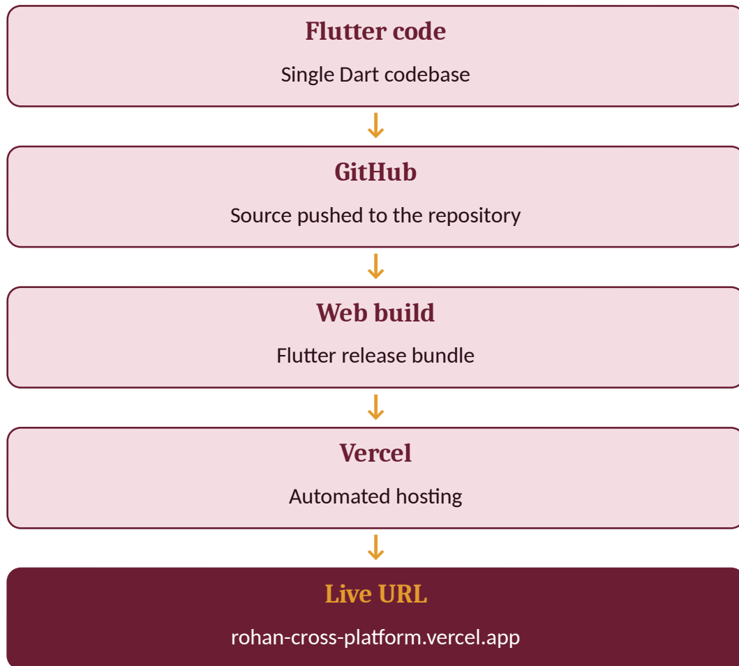
Figure 2: Git to live URL deployment pipeline
