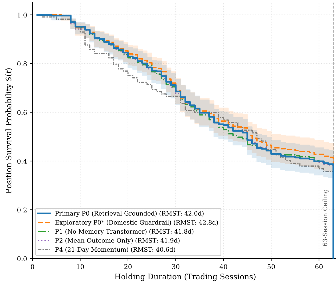
(a) Kaplan-Meier Survival with 95% Greenwood Confidence Bands
