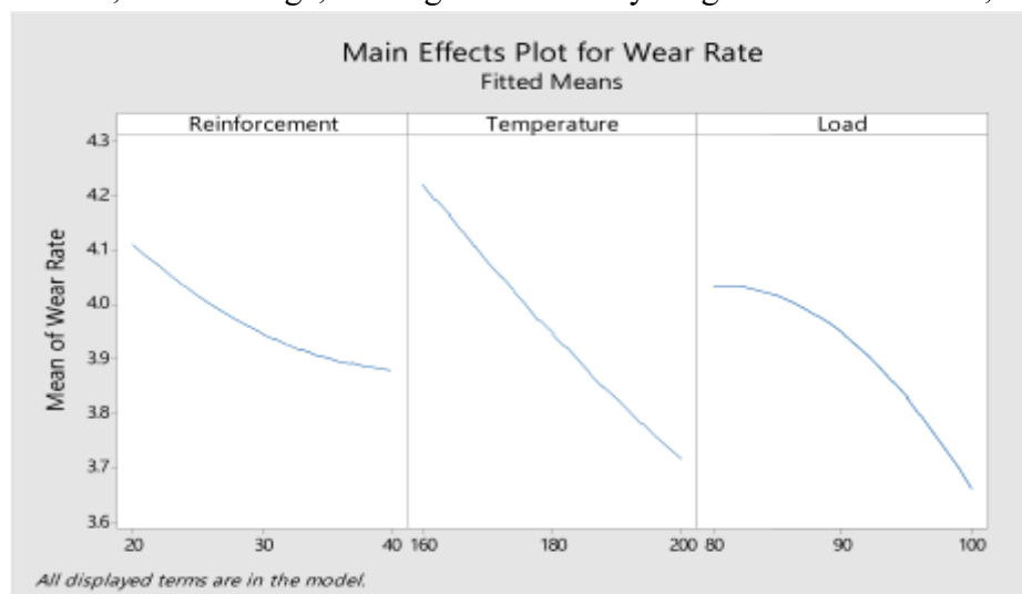
Figure 2 Main Effects Plot of Wear rate.
