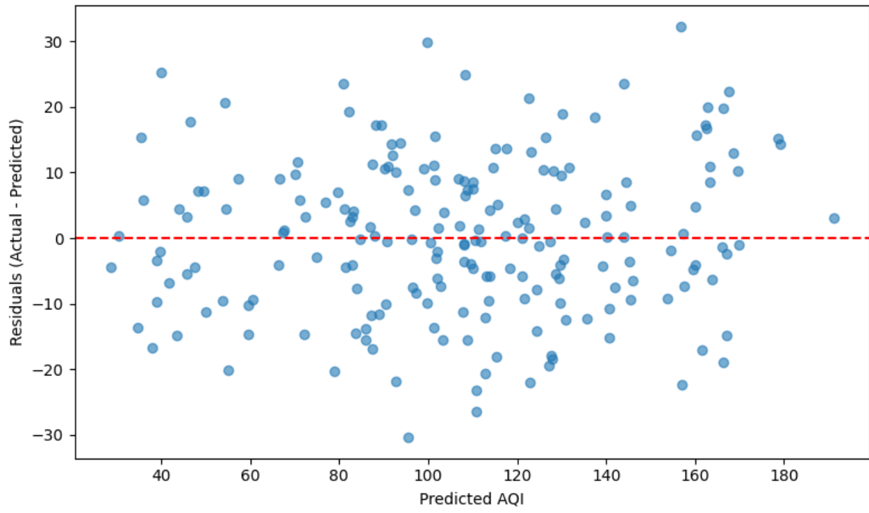
Residuals Plot
