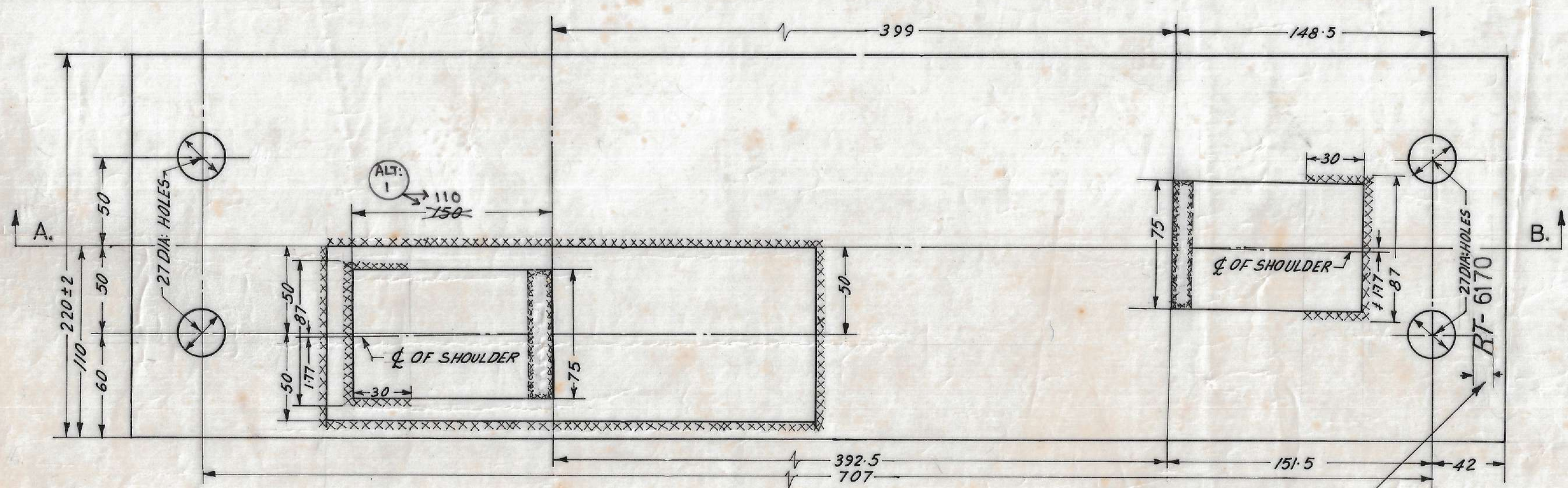
PLAN (AT SLEEPER NUMBER 24)
