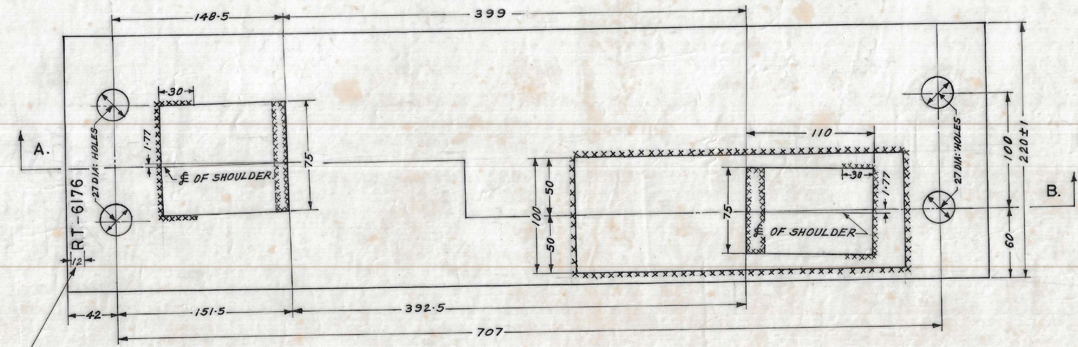
PLAN (AT SLEEPER NO. 24)
