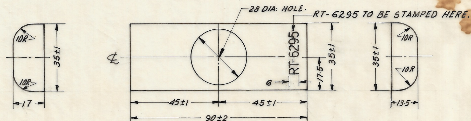
SIDE ELEVATION
