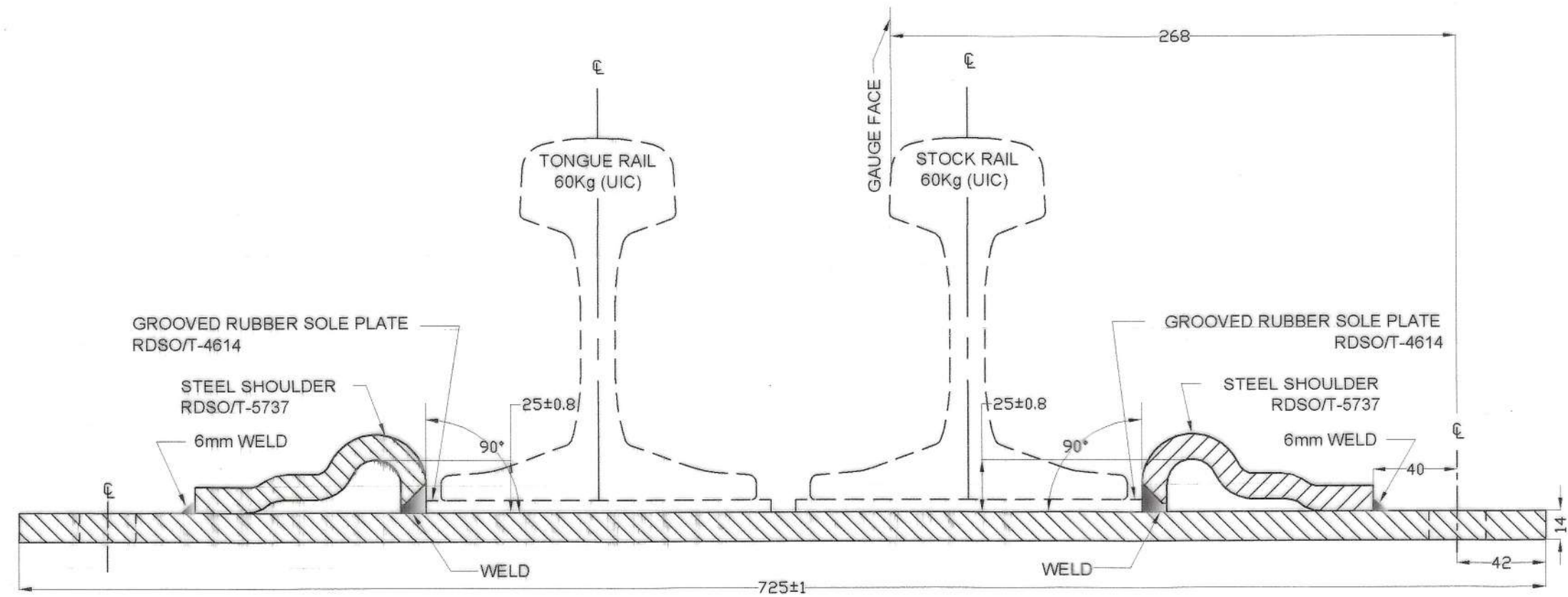
SECTIONAL ELEVATION ON 'AB'
