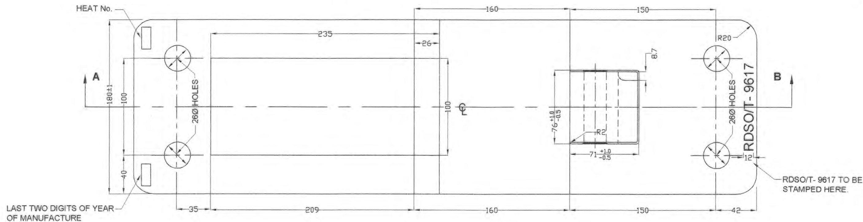
PLAN (AT SLEEPER NO. 21)
