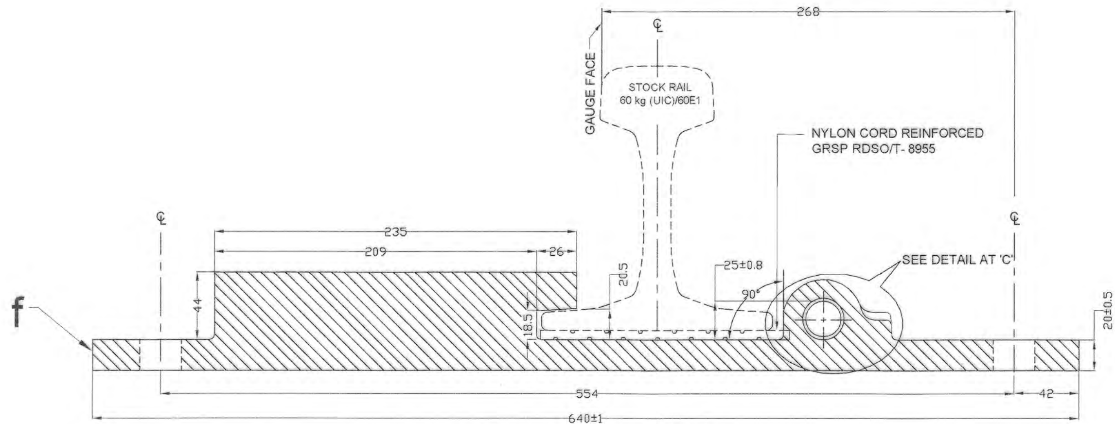
SECTIONAL ELEVATION ON AB
