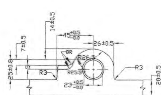
DETAIL 'J'
