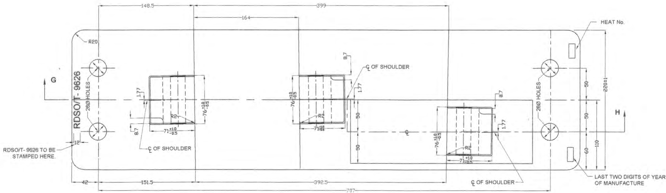
PLAN (AT SLEEPER NO. 24)
