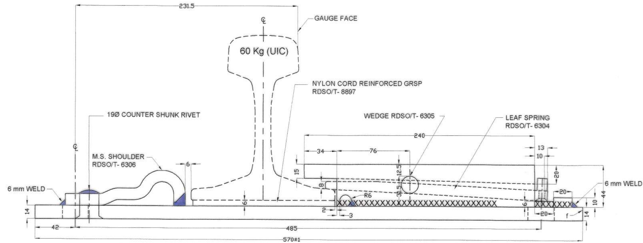
SECTIONAL ELEVATION ON A.B.
