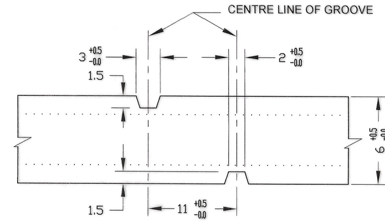
DETAIL OF GROOVES
