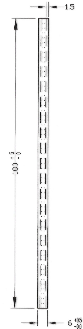
SIDE ELEVATION
