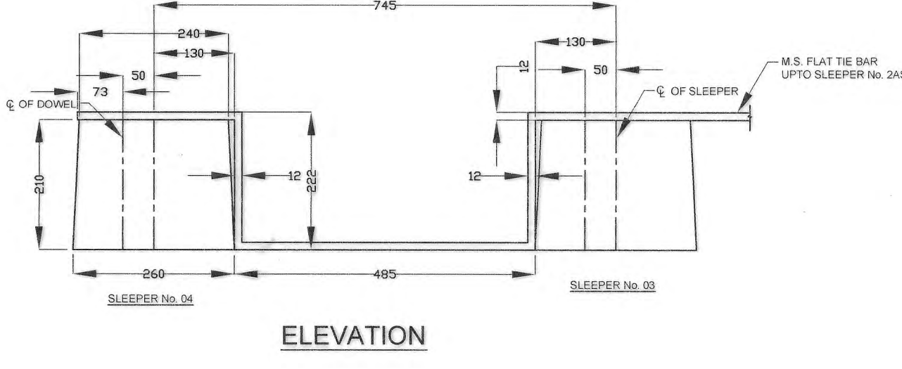
DETAIL 'B' ARRANGEMENT OF M.S. FLAT TIE BAR AT SLEEPER No. 03 & 04
