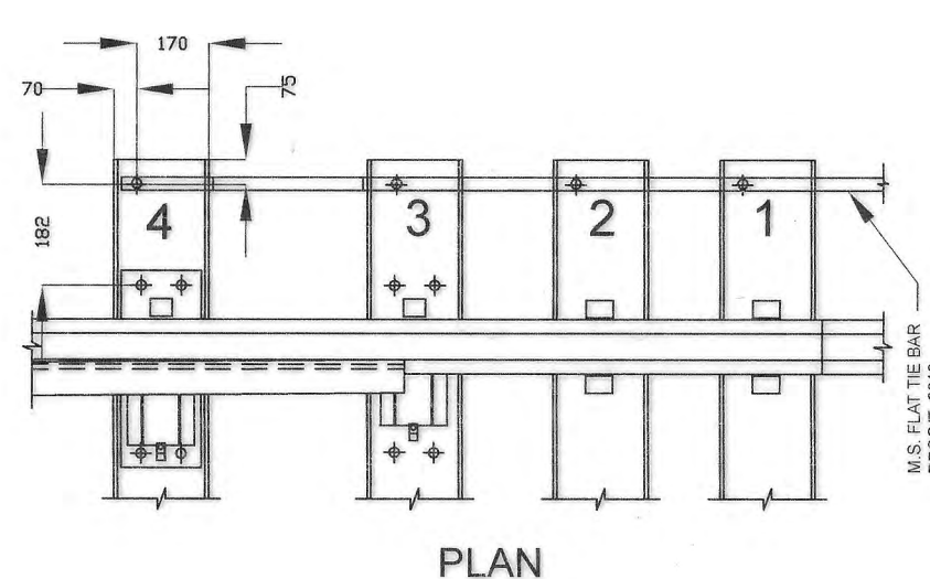
DETAIL 'B' ARRANGEMENT OF M.S. FLAT TIE BAR AT SLEEPER No. 03 & 04
