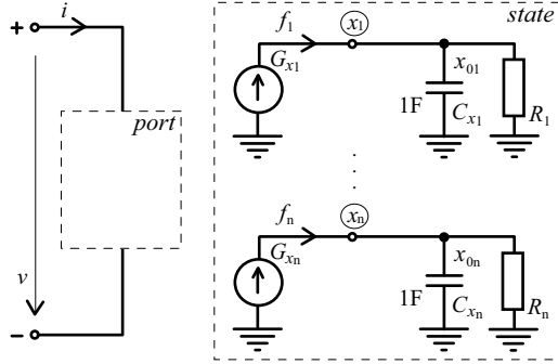
Figure 2. Block diagram of the SPICE model of general n -th order mem-system.
