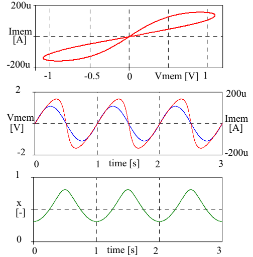
Figure 4. Results of SPICE simulation; HP memristor is driven by a harmonic voltage.
