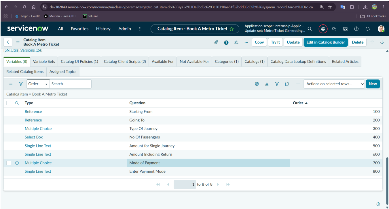
Figure 21. Catalog Item Variables — Book A Metro Ticket
