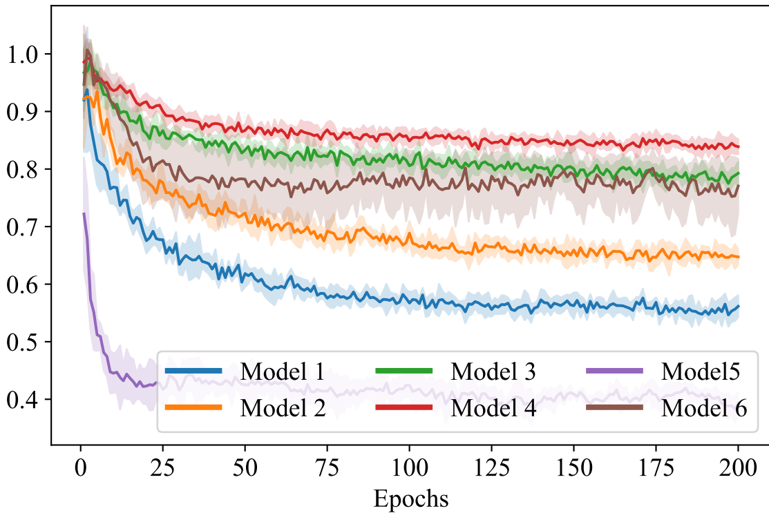
Test/Train Accuracy Ratio
