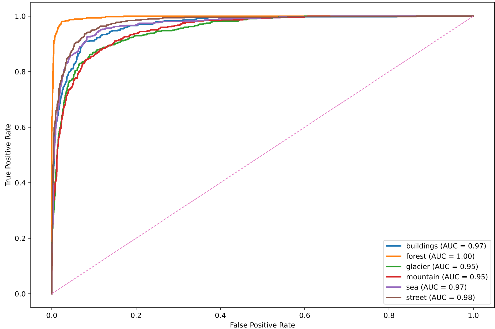
CNN Multi-Class ROC Curve
