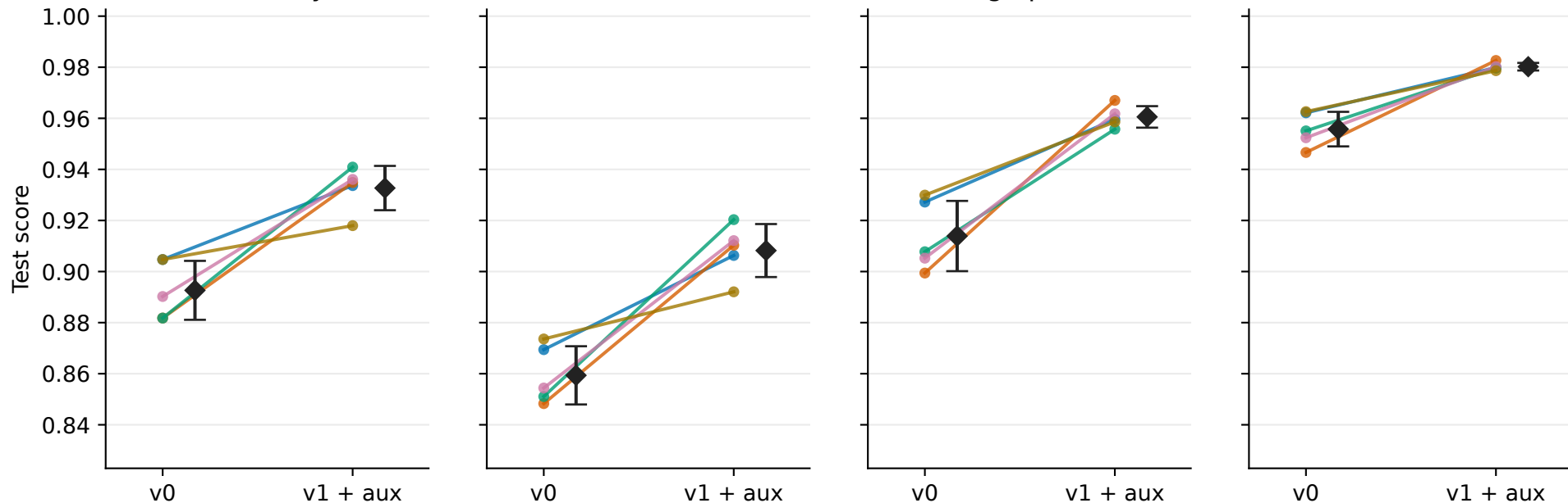
Accuracy
