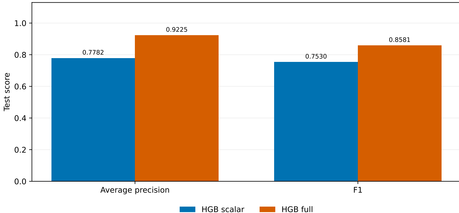
HGB: scalar versus full transit inputs
