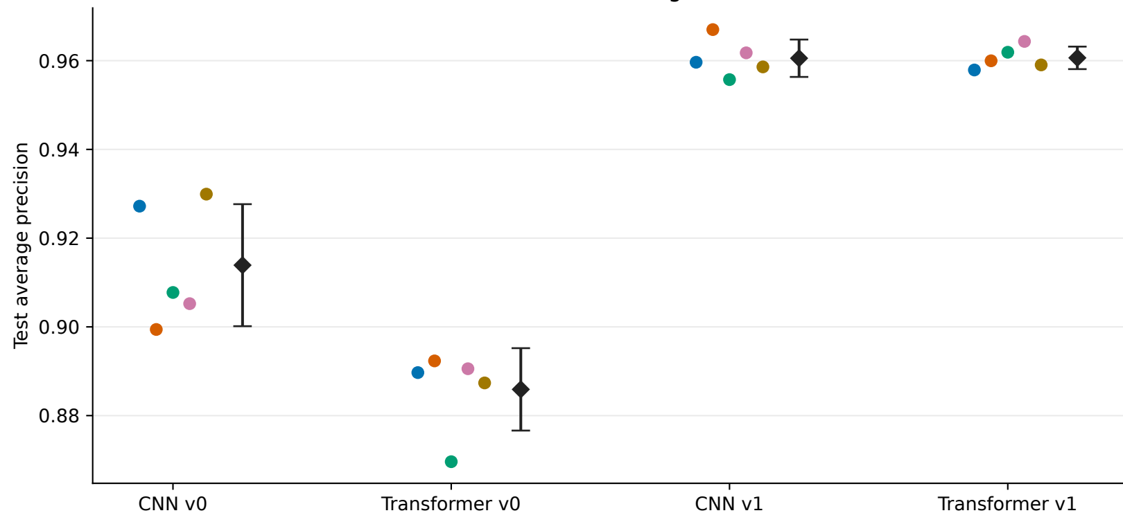
CNN and transformer: existing five-seed results
